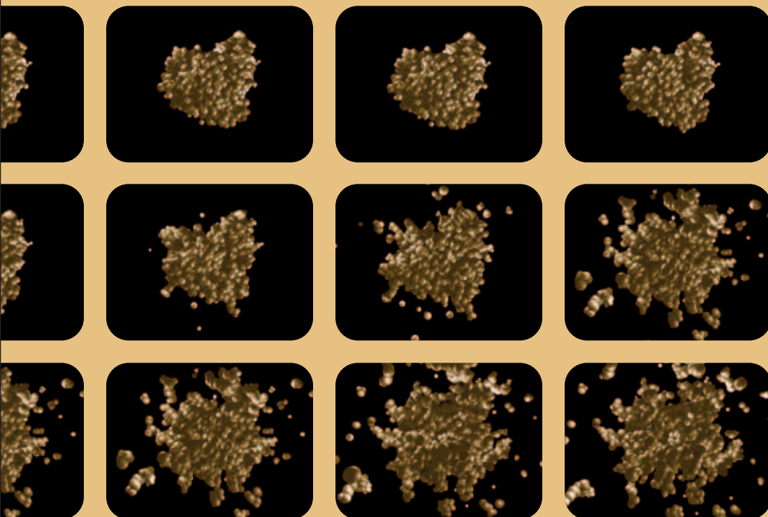
LCLS will use ultra-short, intense x-ray pulses to produce scattering patterns before molecules are destroyed. In this series of images from a simulation, a lysozyme molecule is hit with x-ray light and then explodes. Images: Janos Hajdu, Uppsala Universitet, Sweden
